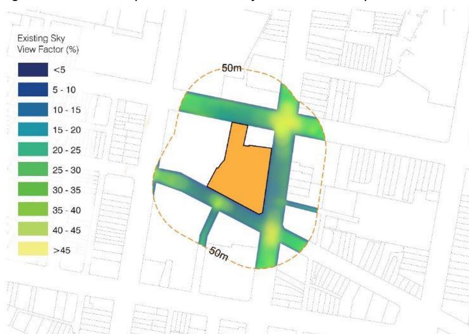
Figure 12.2.12 Example of coloured Sky View Factor map
